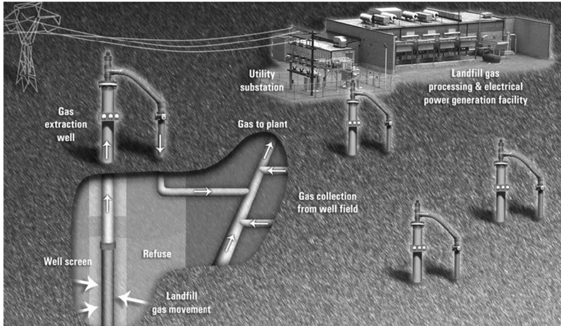
Figure 2: Typical Landfill Gas Collection and Extraction
